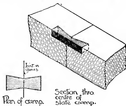
FIG. 11.—(1 in. = 1 ft.)
