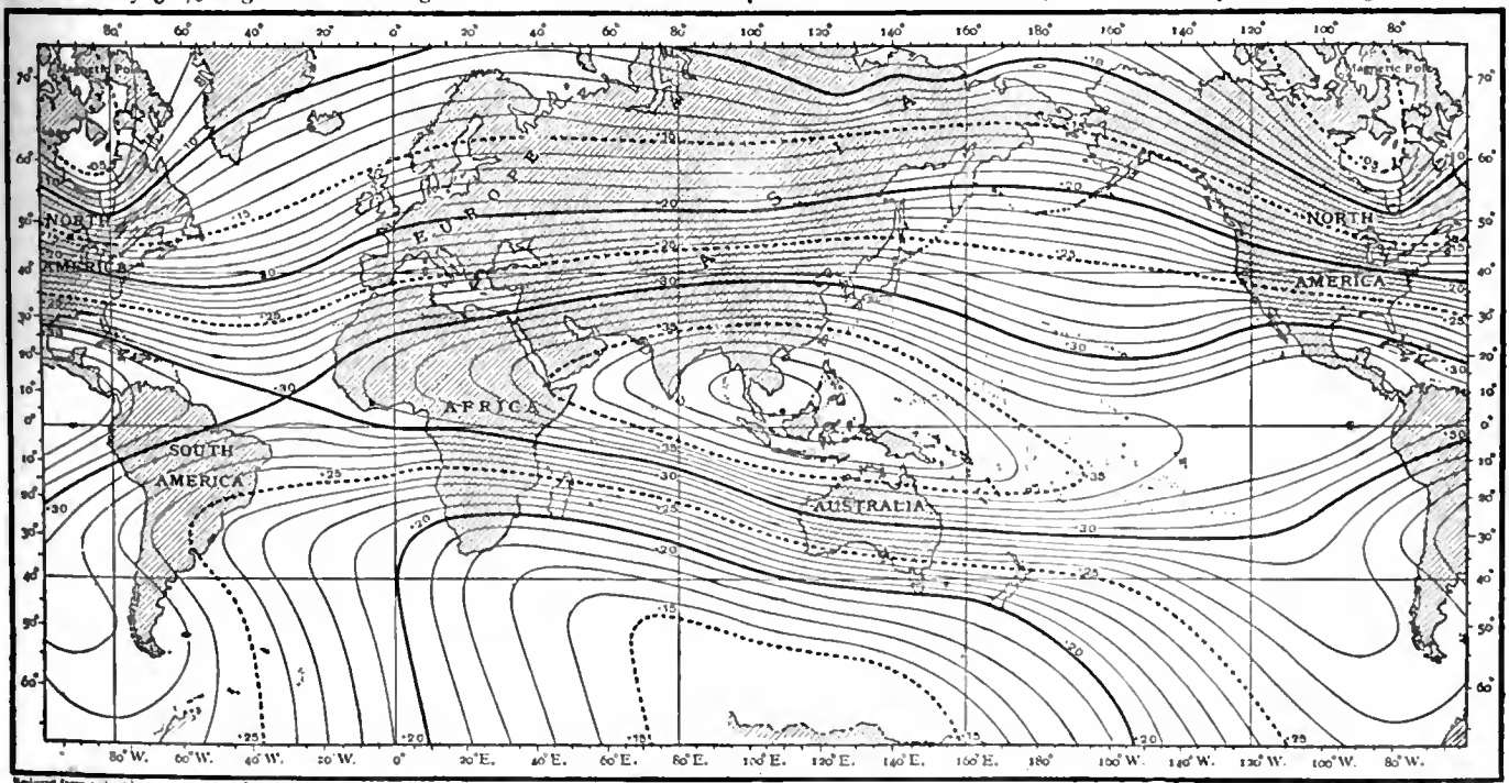
FIG. 3.—Isomagnetics, lines of equal horizontal force.
