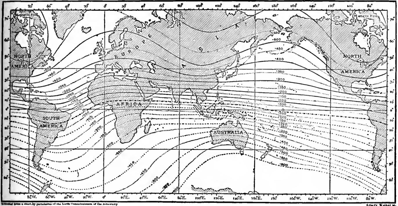
FIG. 2.—Isoclinals, or lines of equal magnetic dip.
