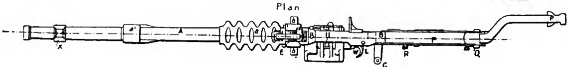
FIGS. 14, 15, 16.—Hotchkiss Gun Mechanism.
