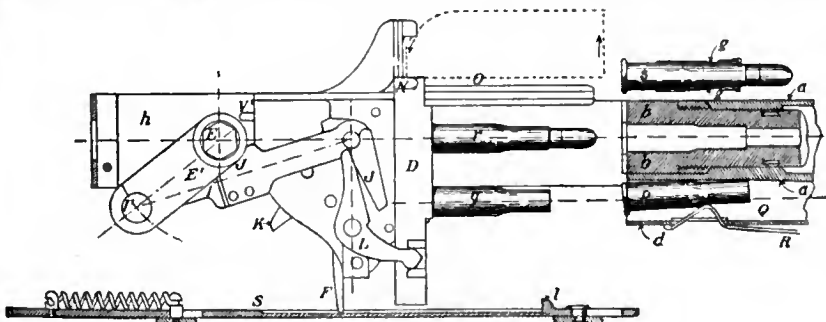
FIG. 10.—Maxim Gun Mechanism.
