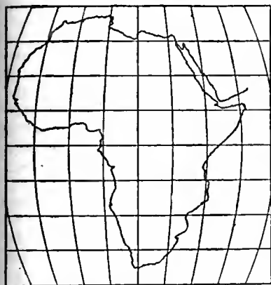
FIG. 19.—Sinusoidal Equal-area Projection.
