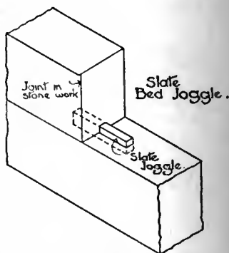
FIG. 12.—(1 in. = 1 ft.)
