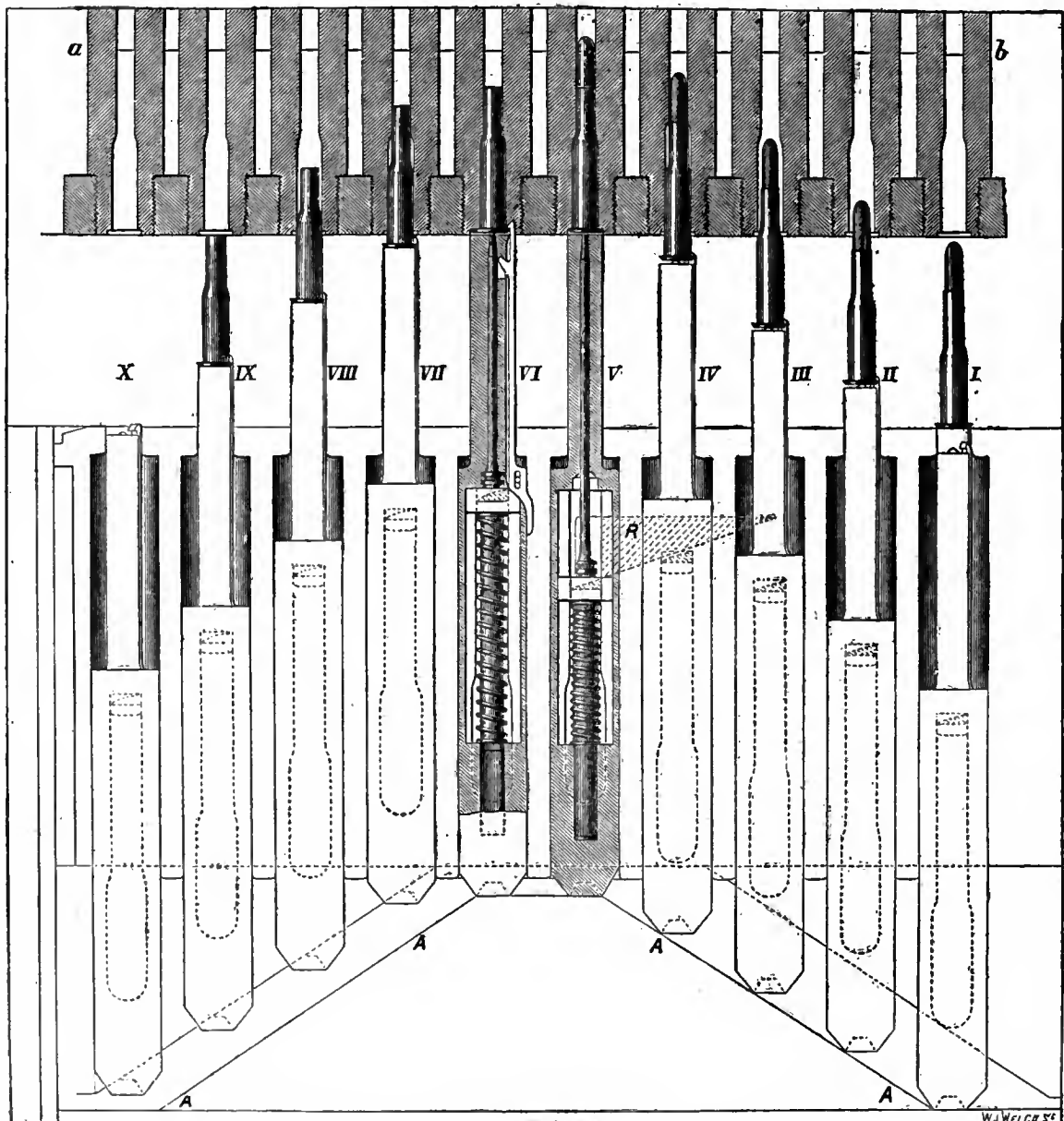
FIG. 4.—Lock of Gatling Gun.
