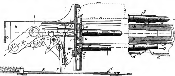
FIG. 12.—Maxim Gun Mechanism.
