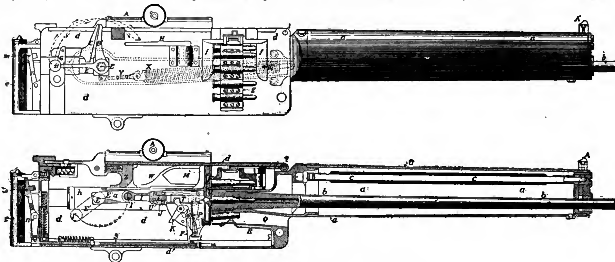
FIGS. 7 and 8.—Mechanism of Maxim Gun.
