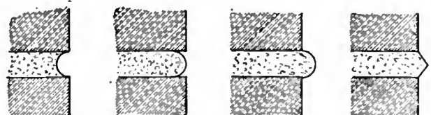
Three forms of Keyed Joints
